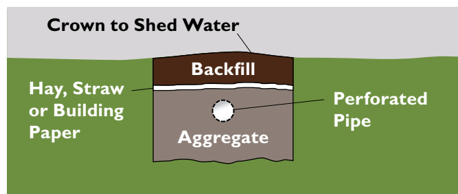
Figure 3: Cross-sectional view through trench
